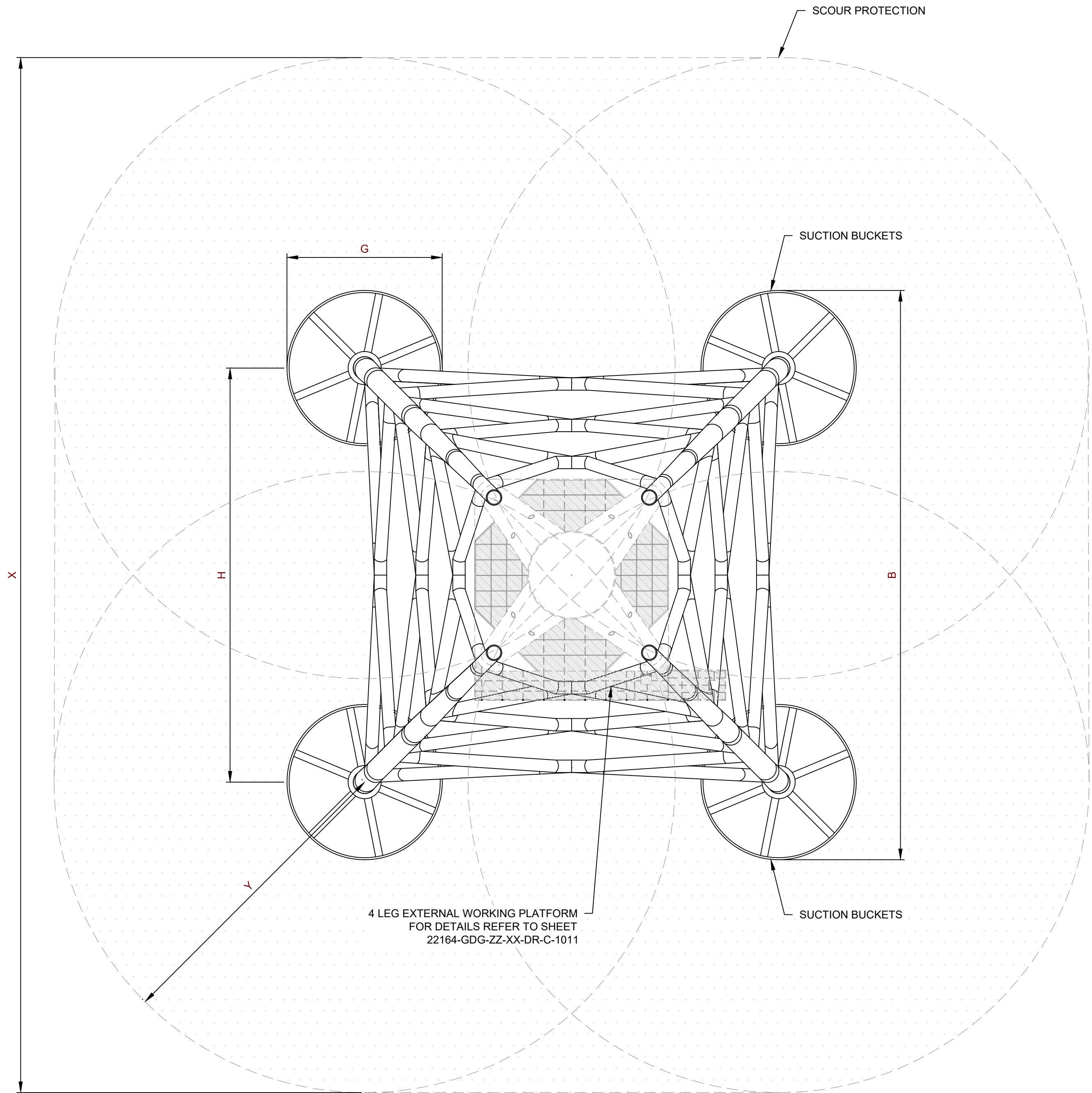
PLAN VIEW - (OPTION A) SCALE 1:300
