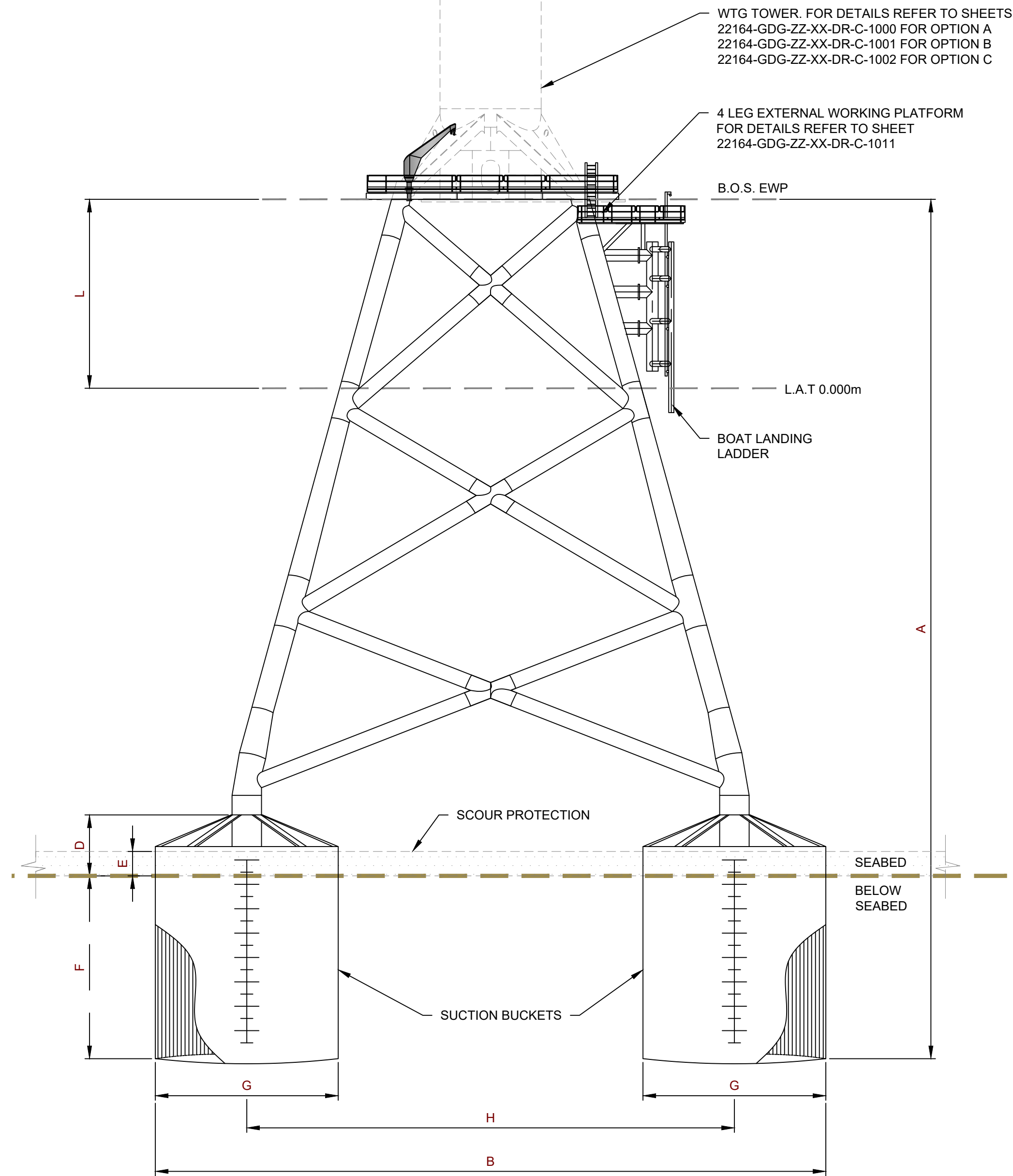
ELEVATION VIEW - (OPTION A) SCALE 1:300
